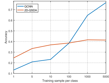
Fig. 9. Comparison of QCNN and 2D-QSDA on CIFAR10.
