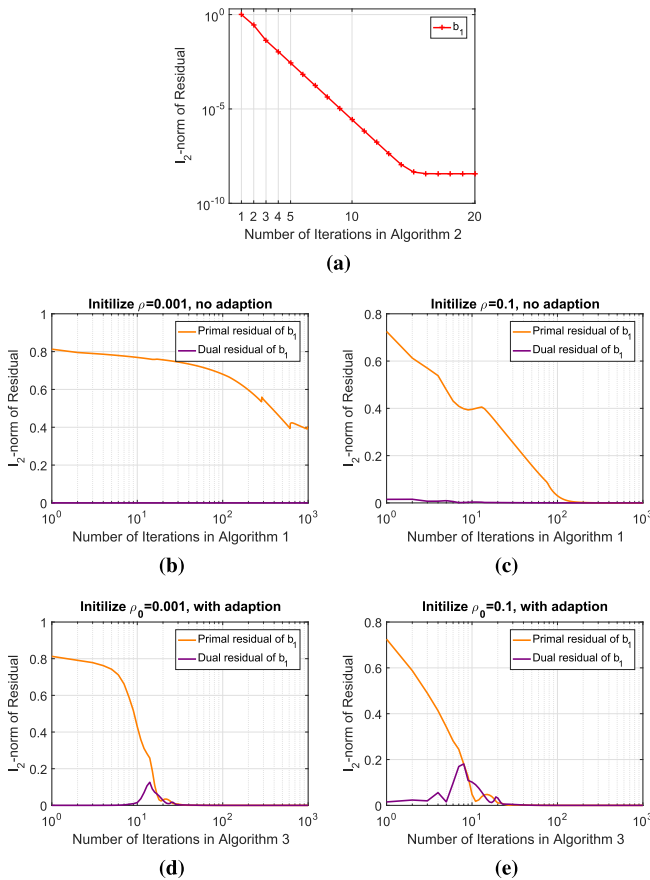
Fig. 1. Empirical convergence of 2D-QSDA: (a) outer iteration; (b) inner iteration with fixed \rho = 0.001 ; (c) inner iteration with fixed \rho = 0.1 ; (d) inner iteration with adaptive \rho and \rho_0 = 0.001 ; (e) inner iteration with adaptive \rho and \rho_0 = 0.1 .
