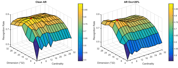
Fig. 6. Classification accuracy vs. cardinality and feature dimension.
