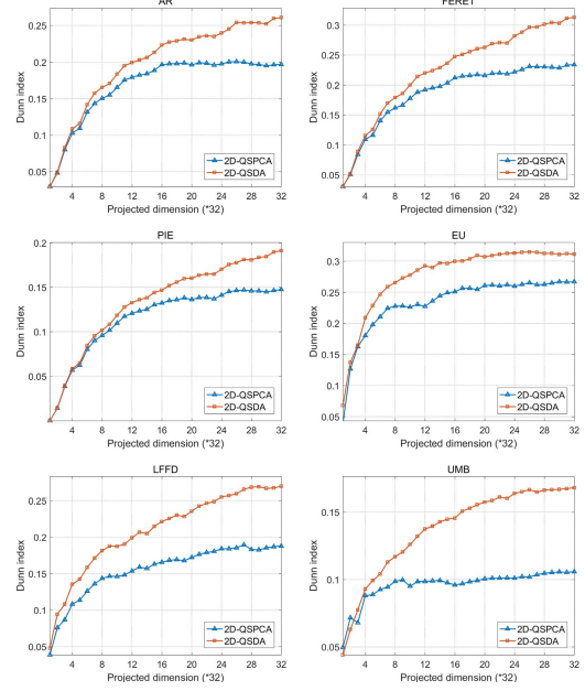
Fig. 8. Comparison of the Dunn index of 2D-QSPCA and 2D-QSDA.
